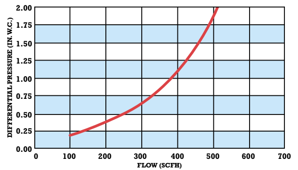
AM-250 PROOF CURVE
